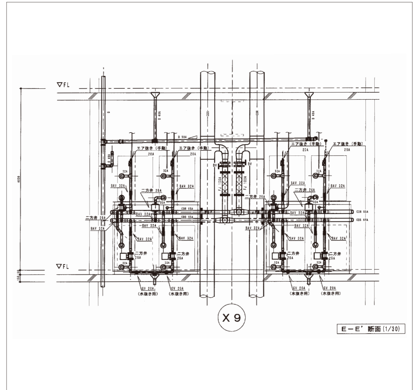
Fig-4 Piping Diagram
