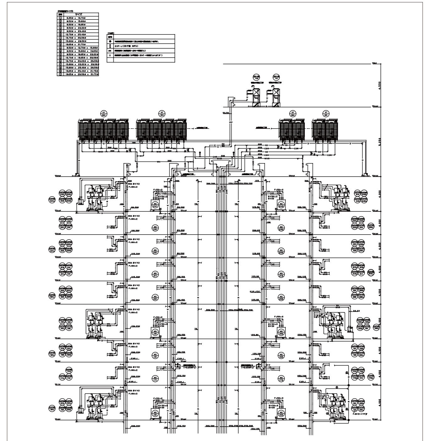
Fig-2 Piping Diagram for VRV Will
