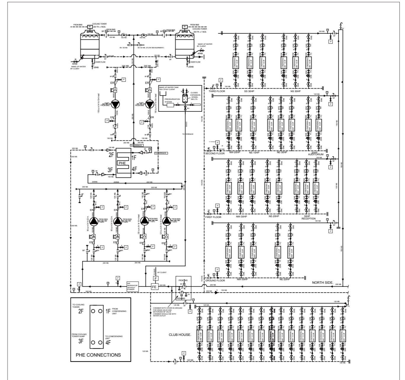
Fig-2 Water Piping Diagram
