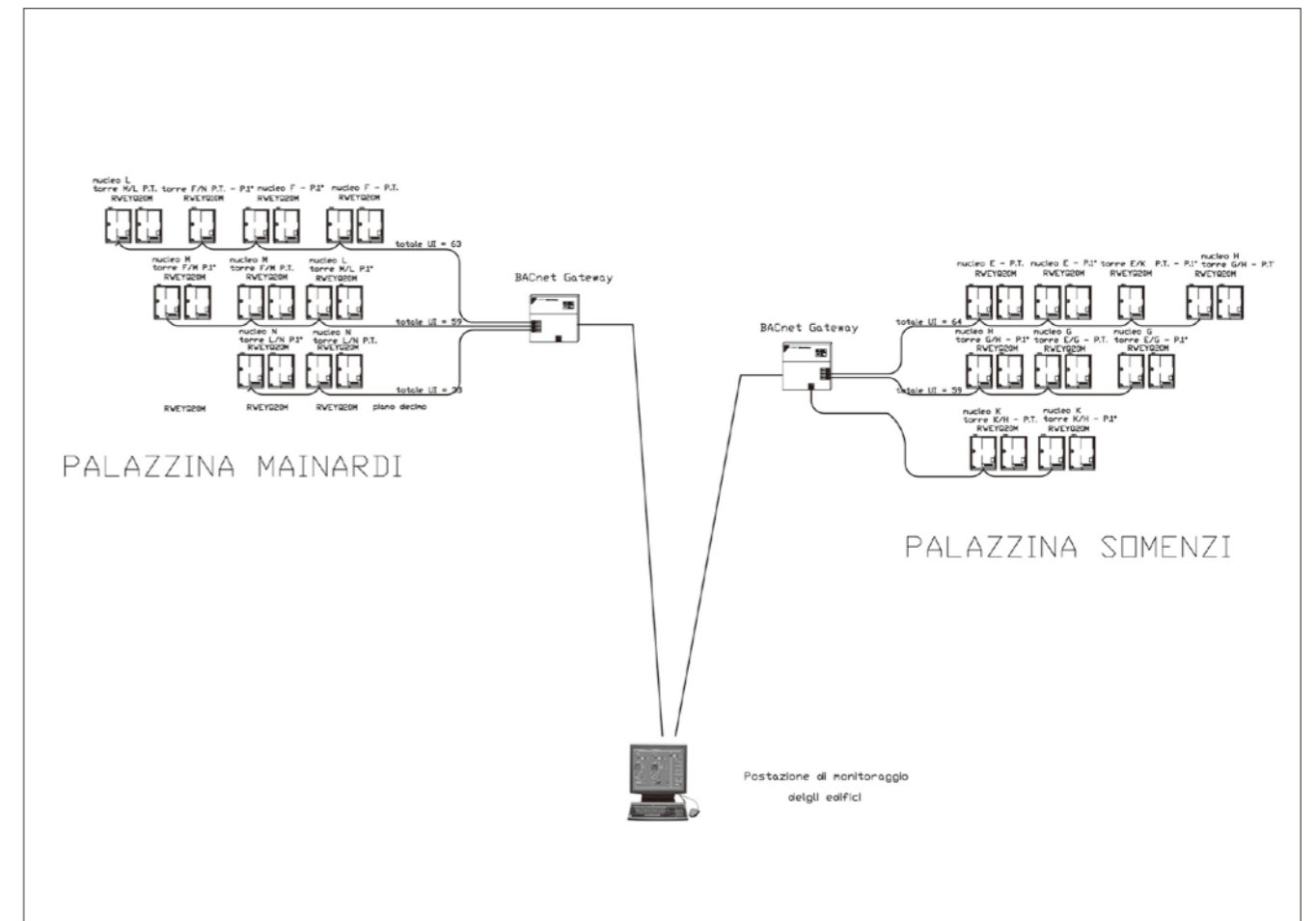
Fig-1 Wiring Diagram
