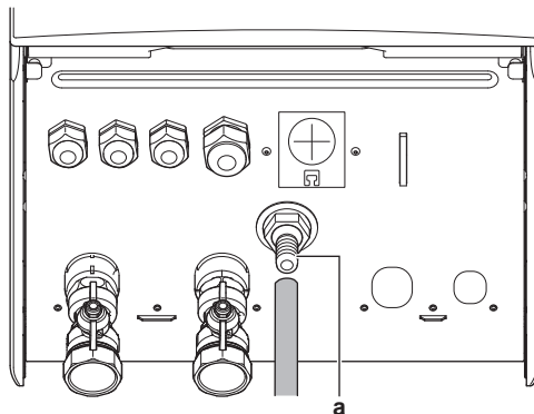
a Lekbakconnector
