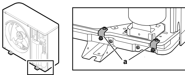
a Transportbeschermers (2×)
